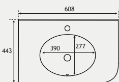
60cm Left Hand Basin
