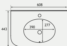
60cm Right Hand Basin
