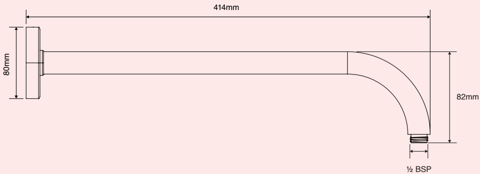
CEILING ARM
