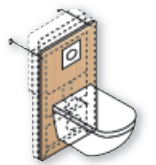
floorstanding wall panel - inc cistern, frame, flush plate & wall hung wc pan 60cm width
