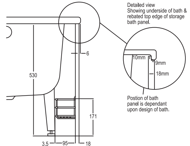
Diagram of a 700mm wide bath, that has legs with a width of 455mm. Panel height 530mm (plus rebate), not trimmable.
