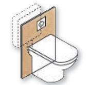
floorstanding wall panel - inc cistern, flush plate & btw wc pan 60cm width
